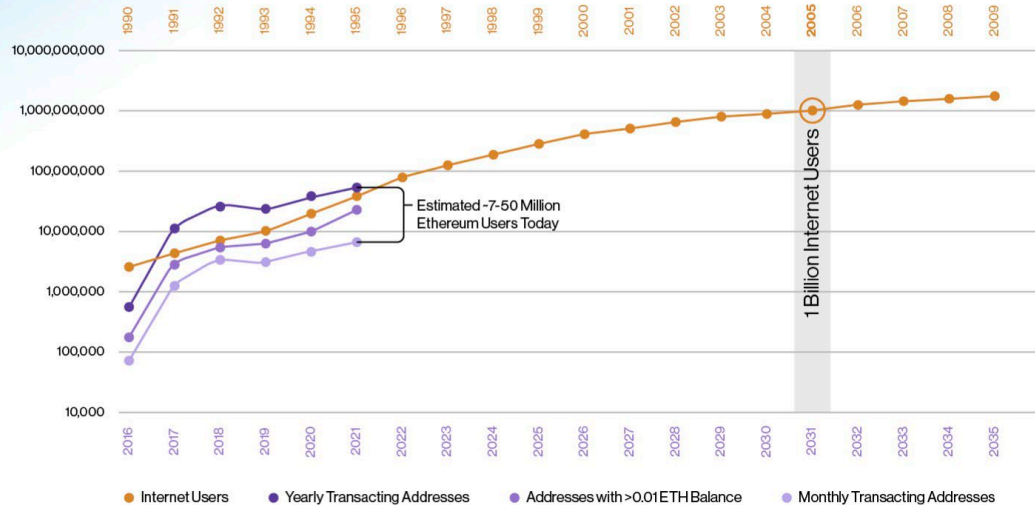
Internet Users vs. Ethereum Addresses (Log Scale)
